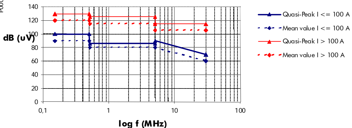
"SECOND ENVIRONMENT" Disturbance Limits
