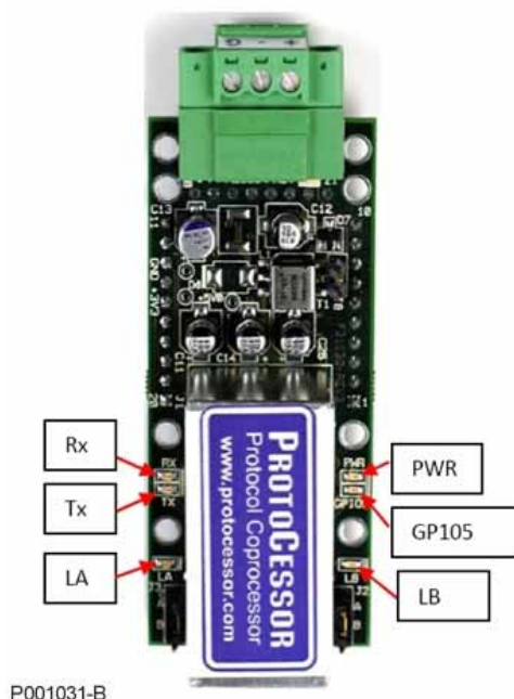
Figura 145: LED IP BACnet
